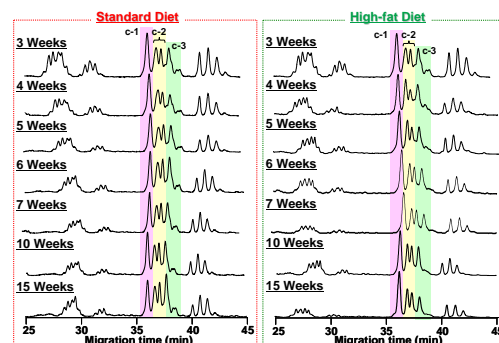
Fig. 2. CE analysis of N-glycans in serum samples of rats raised with standard diet and high-fat diet.
