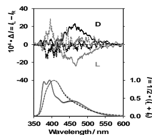
Fig. 2 CPL and PL spectra of Aib3 (solid lines) and 4Py (dotted lines) [D-isomer (black lines) and L-isomer (grey lines)] in EtOH ( 1.0 \times 10^{-4} M).
