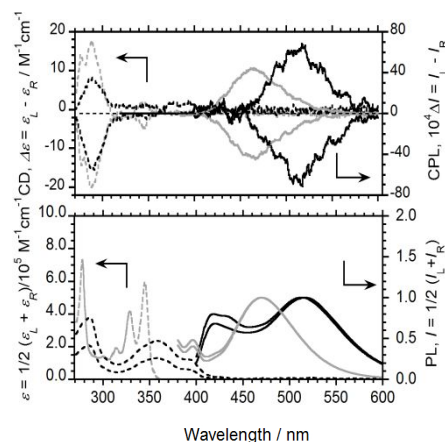
Fig. 1 CD and UV-vis absorption spectra of 1 (gray dotted lines) and 2 (black dotted lines), CPL and PL spectra of 1 (gray lines) and 2 (black lines) in \text{CHCl}_3 (in 1.0 \times 10^{-4} M).
