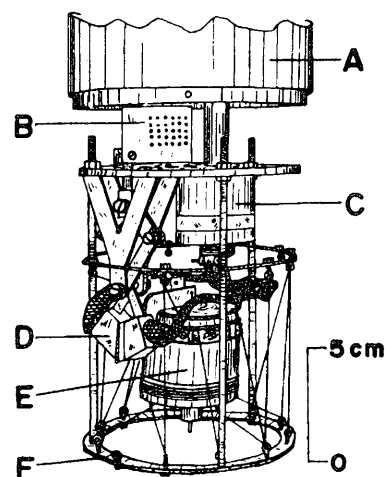
Figure 8 An isoperibol calorimeter for the temperature range 0.3 - 20 K. A, 1.2 K pot ( ^4\text{He} ); B, tag for lead wires; C, ^3\text{He} evaporator (0.3 K); D, mechanical thermal switch; E, calorimeter cell; F, sample mounting flame.
