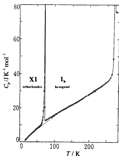
Figure 7 Heat capacity of hexagonal ice I_h doped with KOH in the mole fraction of 10^{-4} .
