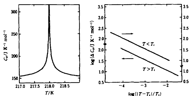
Figure 1 (left) Heat capacity divergence at critical temperature T_c and (right) critical plot of \text{SnCl}_2 \cdot 2\text{H}_2\text{O} single crystal.
