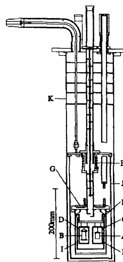
Figure 2 Twin-type adiabatic microcalorimeter. A, sample cell ; B, thermometric block : C and D, inner adiabatic shields : E, outer shield ; F, thermal anchor ; G and H, heat exchangers : I, inner vacuum can : J, radiation shield : K, outer vacuum can
