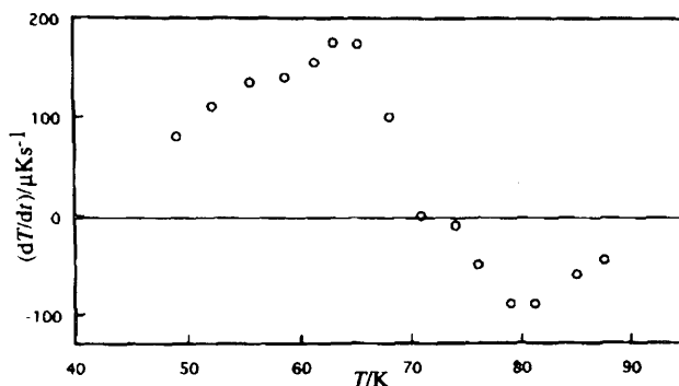
Figure 4 Spontaneous temperature drift rates observed for isopropylbenzene around its secondary ( \beta ) glass transition.
