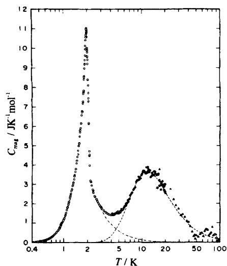
Figure 9 Magnetic heat capacity of ( N,N -diethyldithiocarbamato)-iron(III) iodide.
