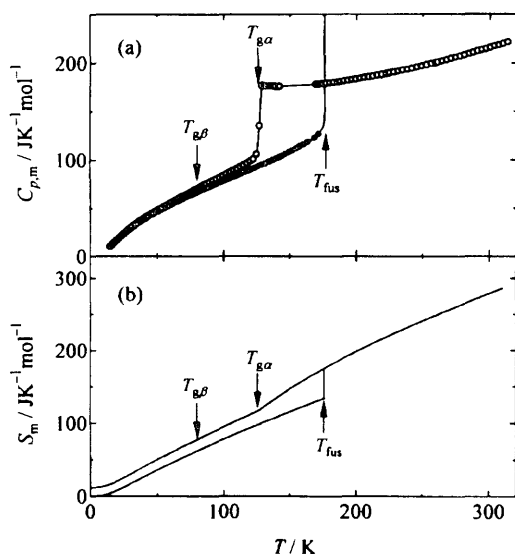
Figure 3 Heat capacity of isopropylbenzene. T_{g\alpha} and T_{g\beta} are primary and secondary glass transitions of the liquid.
