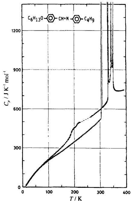
Figure 6 Heat capacity of p-n -hexyloxybenzylidene- p' -butylaniline.
