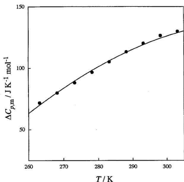
Figure 5. Excess heat capacity of 1:1 complex over that of 1:1 mechanical mixture
