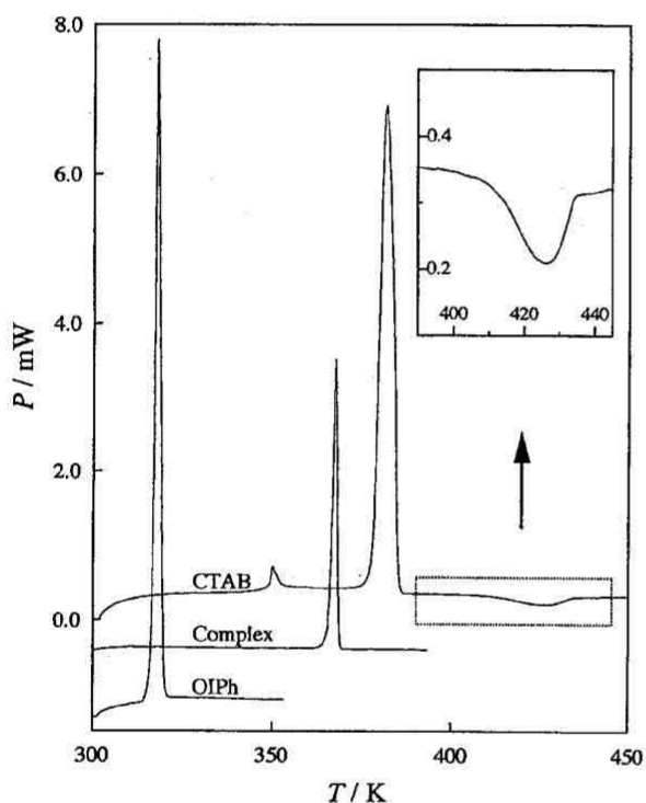
Figure 1. DSC curves of CTAB, 1:1 complex, and OIPh. The high temperature part of CTAB crystal is reproduced in the inset in a magnified scale.
