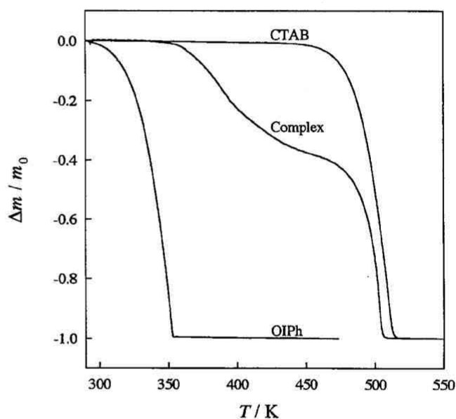
Figure 2. TG curves of CTAB, 1:1 complex, and OIPh.
