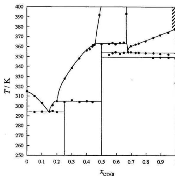
Figure 4. Phase diagram of CTAB-OIPh binary system.
