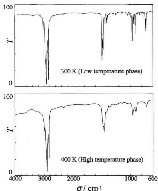
Figure 3. IR spectra of CTAB crystal taken at 300 K (low-temperature phase) and 400 K (high-temperature phase).
