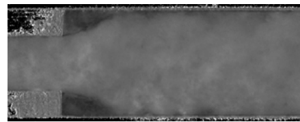
(a) 低流速 ( U_a=0.06\text{ m/s} )
